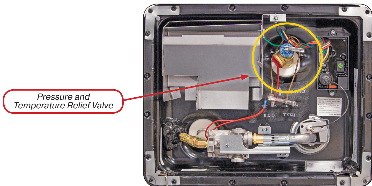
Inside the Exterior Water Heater Door
