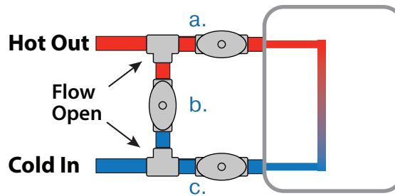
Draining the Water Heater - Valve Positions
