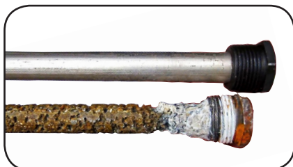
Brand New Anode Rod (top) Corroded Anode Rod (bottom)
