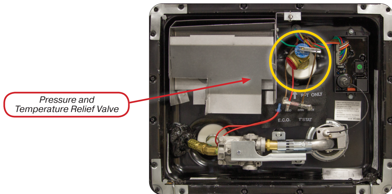
Exterior Water Heater Door
