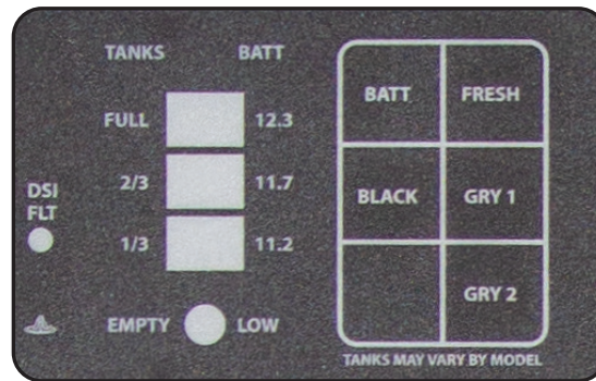
Monitor Panel
