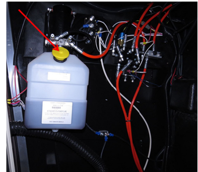
Typical reservoir for both the hydraulic landing gear and hydraulic slide system, it is located in the front-facing compartment. The red arrow points to the breather/fill cap.
