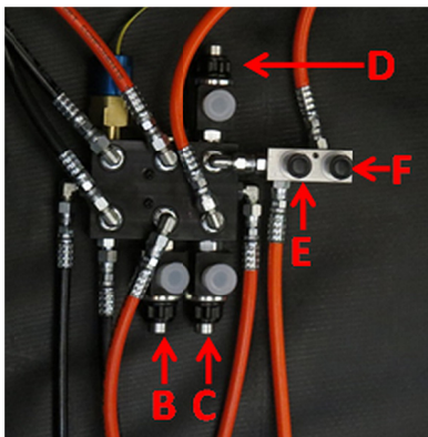
Typical hydraulic slide rooms and leveling legs override valves, generally located in the front facing compartment.
