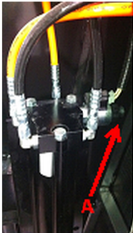
Typical hydraulic front landing legs override valve, generally located in the front, door-side compartment.
