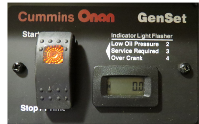
Typical generator remote START/STOP control, located inside the Command Center.
