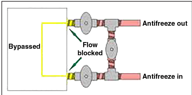
Water heater bypass 3-valve system:
