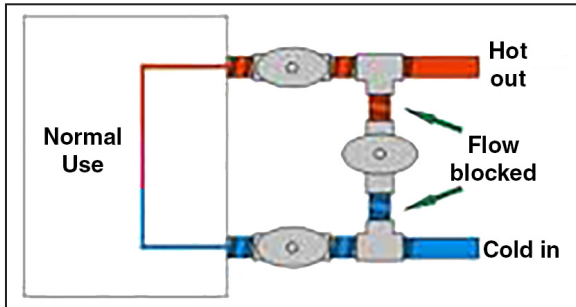
Water heater bypass 3-valve system:
